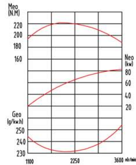
Full speed & full load characteristic curve Model QD32T diesel engine
