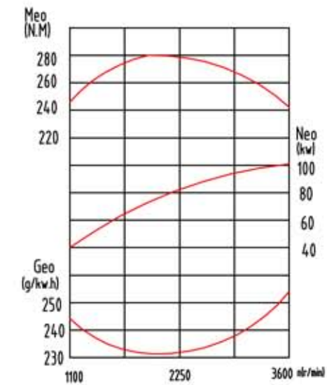
Full speed & full load characteristic curve Model QD32Ti diesel engine
