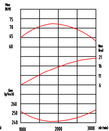
Full speed & full load characteristic curve Model 380 diesel engine
