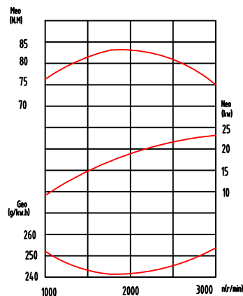
Full speed & full load characteristic curve Model 385 diesel engine
