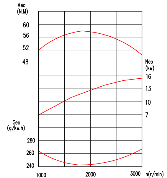
Full speed & full load characteristic curve Model 3M78 diesel engine
