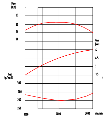
Full speed & full load characteristic cure Model JD500 diesel engine
