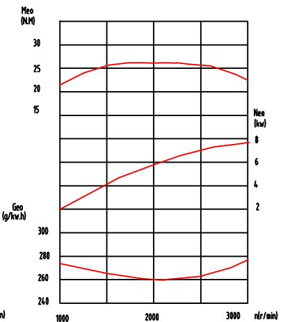
Full speed & full load characteristic cure Model JD550 diesel engine
